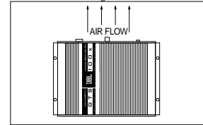
GOOD-Horizontal Mounting
